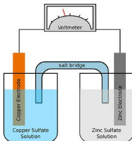
Galvanic cell
