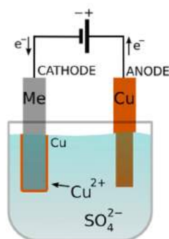
Fig: Process of electroplating
